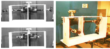
Fig. 5. The humanoid robot Dexter in its start and goal configurations (left) and enacting a successful motion plan (right)
